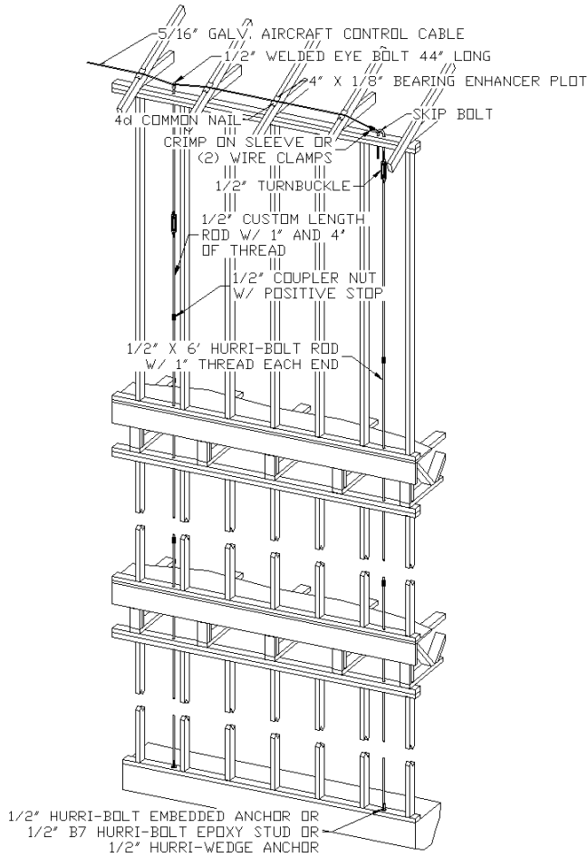
FIGURE 1 HURRI-BOLT TRUSS TIE DOWN SYSTEM
