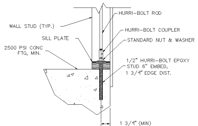
FIGURE 6 HURRI-BOLT EPOXY ANCHOR - HBE (1/2 inch Diameter Shown)
