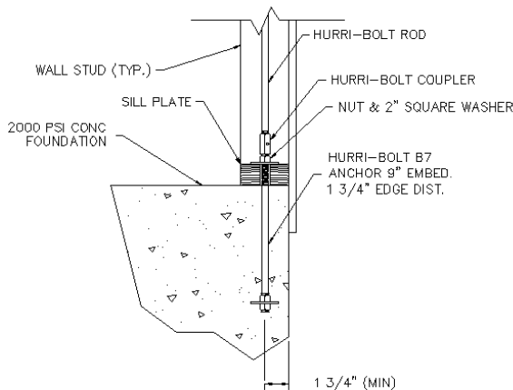
FIGURE 3 HURRI-BOLT CAST IN PLACE ANCHOR
