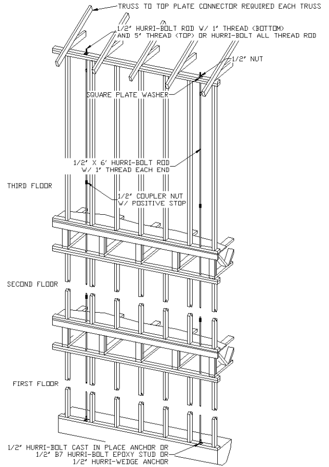
FIGURE 2 HURRI-BOLT TOP PLATE TIE DOWN SYSTEM (1/2 inch Diameter Shown)
