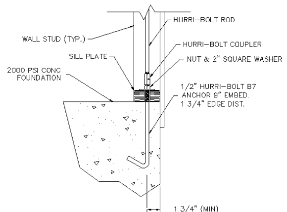
FIGURE 4 HURRI-BOLT ALTERNATE CAST IN PLACE ANCHOR -HBA (1/2 inch Diameter Shown)
