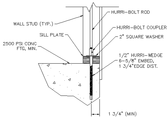
FIGURE 5 HURRI-WEDGE ANCHOR - HW (1/2 inch Diameter Shown)
