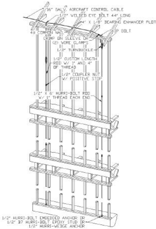
FIGURE 3 HURRI-BOLT CAST IN PLACE ANCHOR
